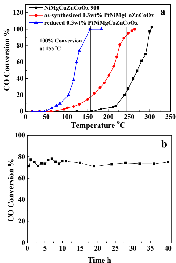
Figure 4. (a) CO oxidation activity of 0.3wt%PtNiMgCuZnCoO x synthesized by co-precipitation. (b) CO oxidation activity of reduced 0.3wt%PtNiMgCuZnCoO x synthesized by co-precipitation upon reaction time under reaction temperature of 135 °C. Reaction condition: a catalyst loading of 20 mg, a flow rate of 12.5 mL/min, and 1 vol % CO balance in air.
