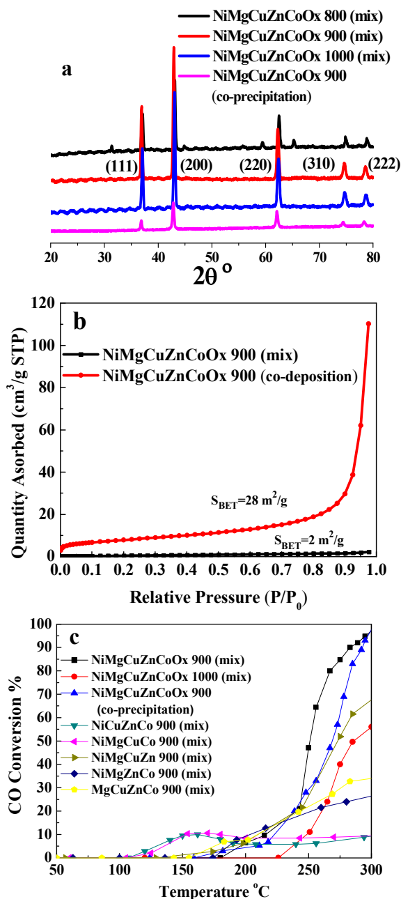
Figure 1. (a) X-ray diffraction patterns for NiMgCuZnCoO x ; (b) Nitrogen adsorption-desorption isotherms of NiMgCuZnCoO x synthesized by physical mixture and co-precipitation method. (c) CO oxidation activity of NiMgCuZnCoO x synthesized by physical mixture and co-precipitation method. Reaction condition: a catalyst loading of 20 mg, a flow rate of 12.5 mL/min, and 1 vol % CO balance in air.
