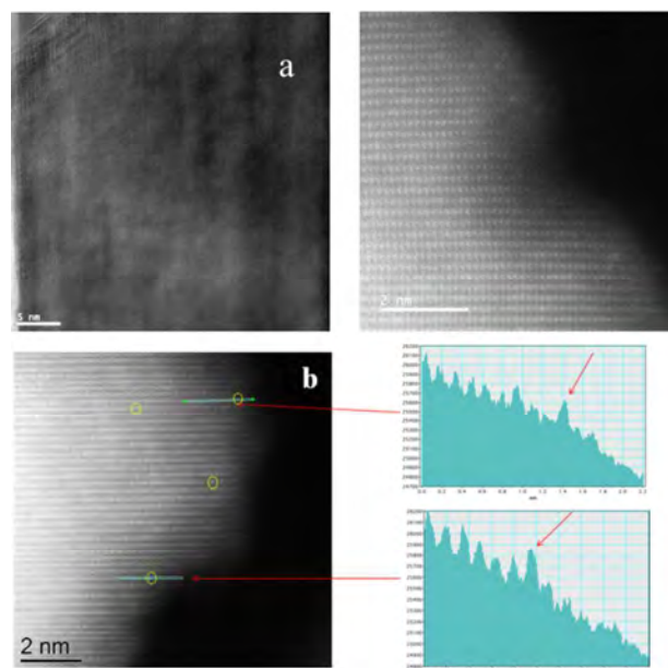
Figure 3. TEM and HAADF-STEM images of reduced 0.3wt%PtNiMgCuZnCoO x .
