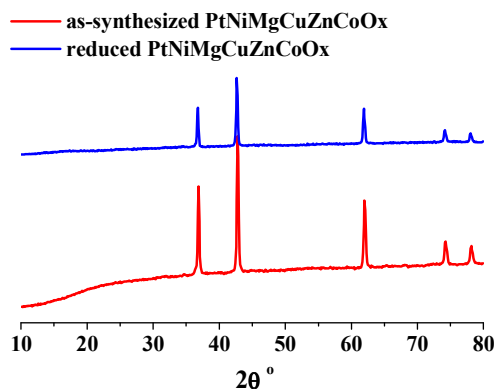
Figure 2. X-ray diffraction patterns for as-synthesized and reduced 0.3wt%PtNiMgCuZnCoO x synthesized by co-precipitation.
